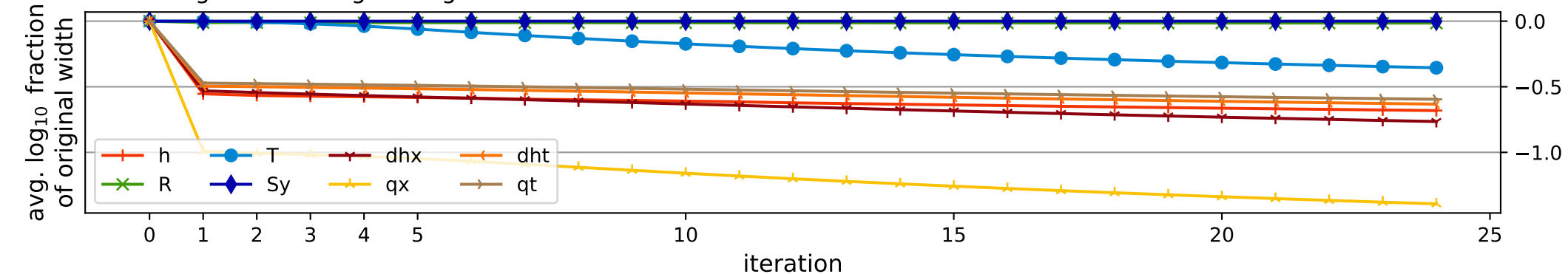
E: Average variable tightening
