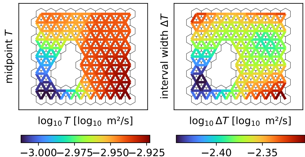
B: Transmissivity
