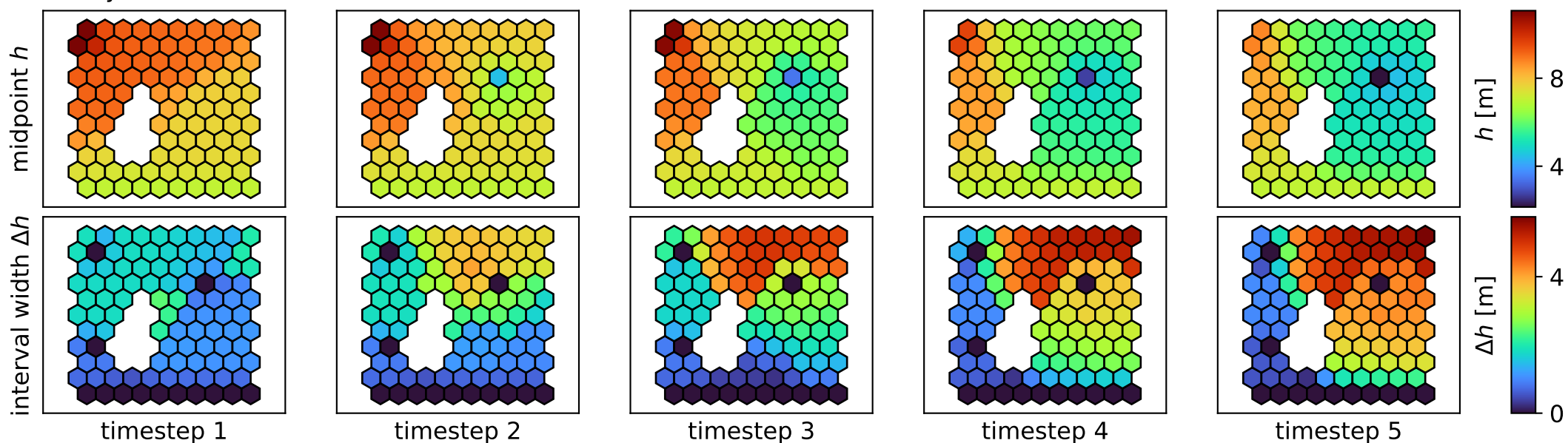
D: Hydraulic head
