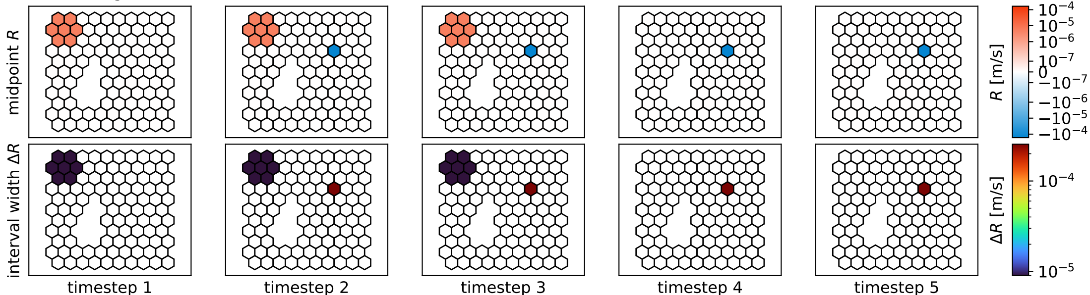
C: Recharge
